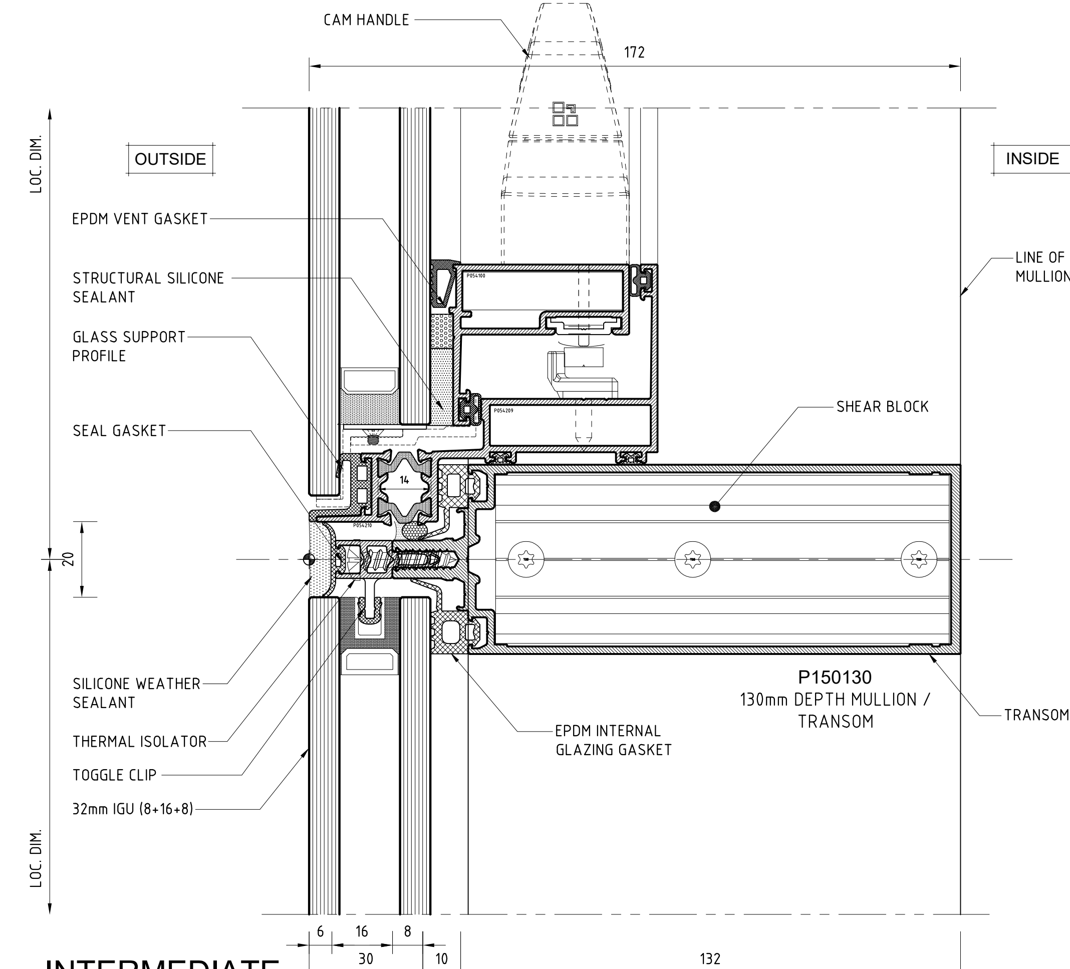
INTERMEDIATE TRANSOM DETAIL
