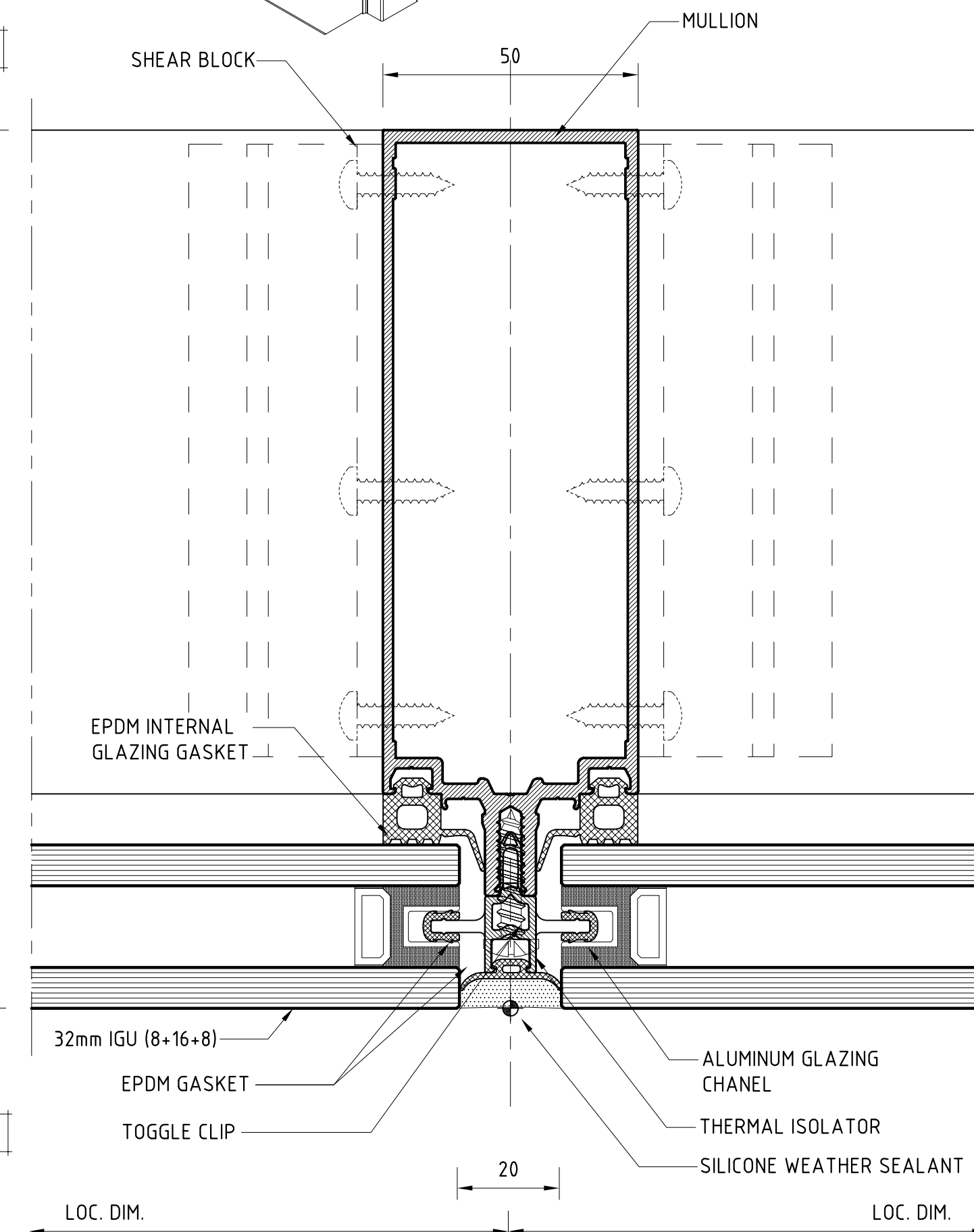
INTERMEDIATE MULLION DETAIL
